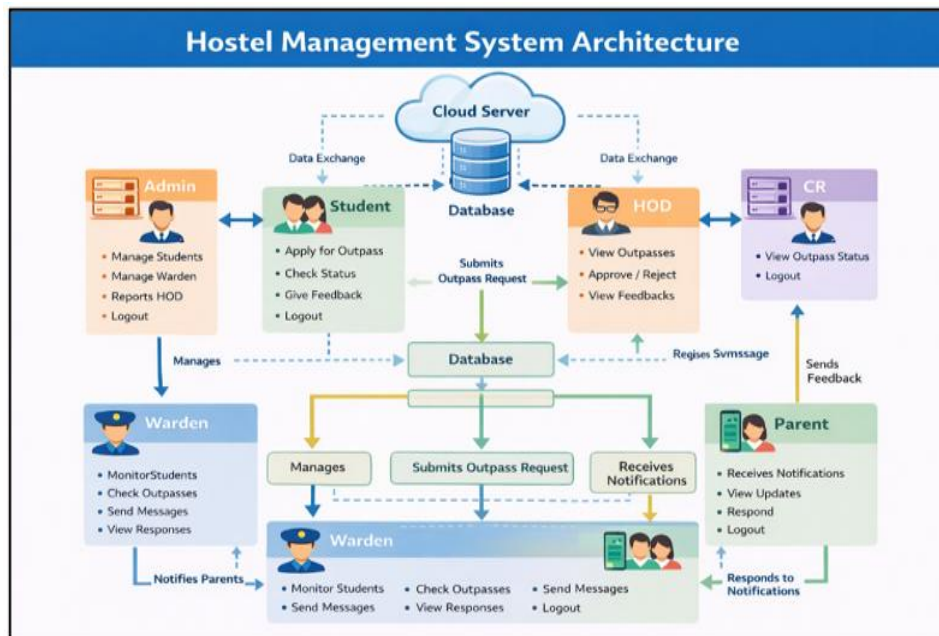
Figure 2 Architecture
