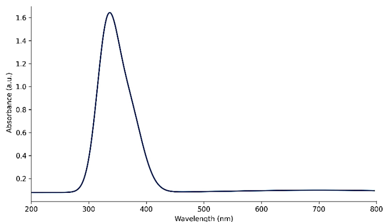
Figure 3. UV-VIS spectrum of CuO–CeO 2 nanocomposite
