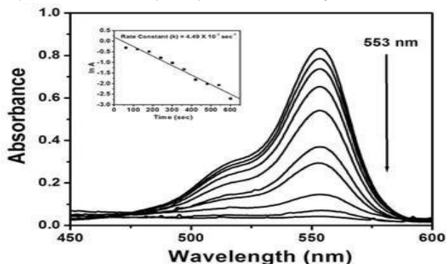
Figure 13: Using AuNPs made from S. tenerimum , Rhodamine B may be reduced catalytically at 553 nm using the UV-visible
