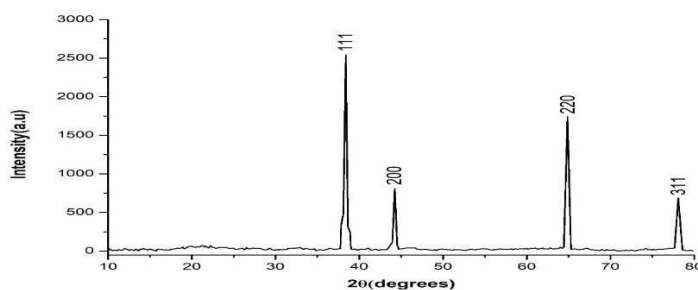
Figure 3: XRD patterns of AuNPs using S. tenerrimum extract
