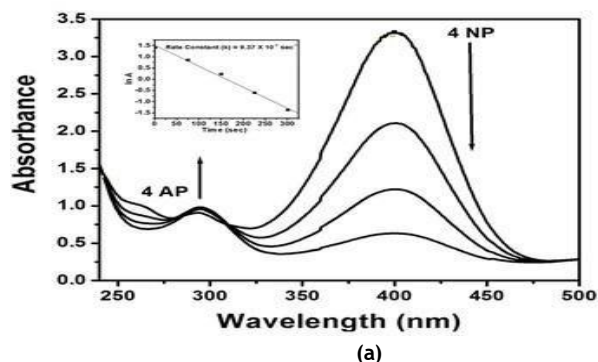
Figure 12: When 4-NP and p-NA were reduced by borohydride using AuNPs from S. tenerrimum as the catalyst, a time-dependent UV-visible spectrum was obtained (a, b). The proper kinetic plots of ln A (A = absorbance of a 4-nitrophenolate ion at 400 nm) vs. time are shown in the inset
