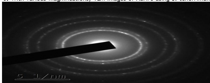
Figure 7: SAED pattern of AuNPs using S. tenerrimum extract
