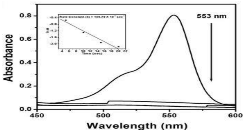
Figure 13: Using AuNPs made from S. tenerimum , Rhodamine B may be reduced catalytically at 553 nm using the UV-visible
